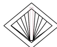
ROMBAS
